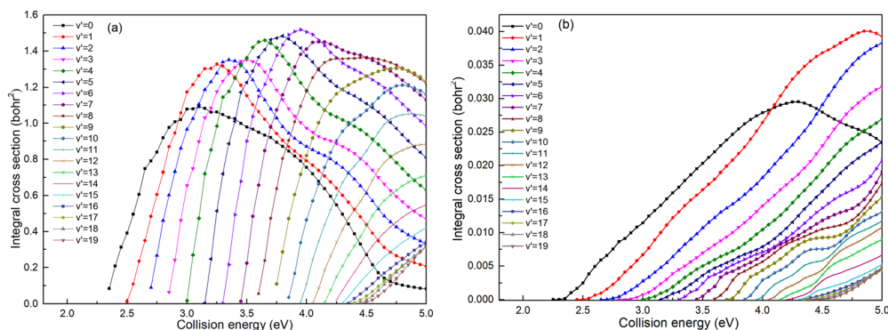
Fig. 7 Vibrational state-resolved ICSs of the \text{Ca}^+(4s^2\text{S}) + \text{H}_2(\text{X}^1\Sigma_g^+) \rightarrow \text{H}(\text{S}) + \text{CaH}^+(\text{X}^1\Sigma^+) reaction calculated based on the adiabatic PES (a) and non-adiabatic PES (b).
