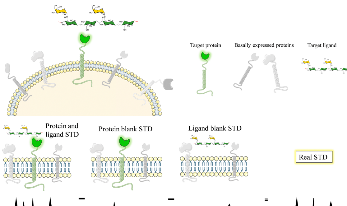
Fig. 24 Scheme of the protocol to carry out on-cell NMR experiments.
