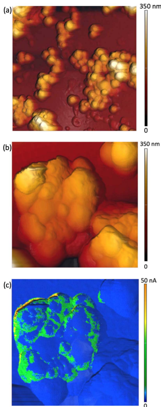
Fig. 4 AFM images of Sepia-PVB films: (a) 3\ \mu\text{m} \times 3\ \mu\text{m} -sized, (b) 1\ \mu\text{m} \times 1\ \mu\text{m} -sized and (c) current image corresponding to the AFM image in (b).
