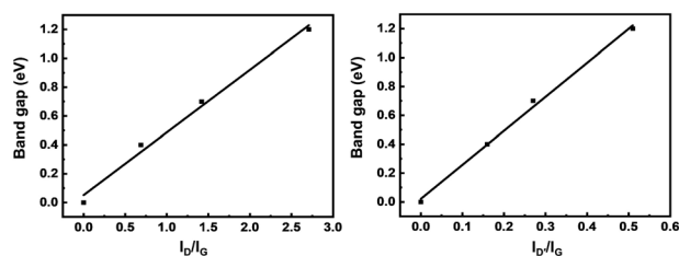
Fig. 4 Band gap of SLG/SLGBr/SLG diodes with different degrees of bromination vs. (a) I_{\text{D}}/I_{\text{G}} and (b) I_{\text{D}}'/I_{\text{G}}' , respectively.
