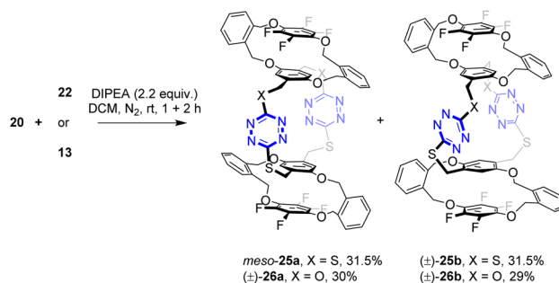
Scheme 5 Synthesis of bispiropanes 25 and 26 .
