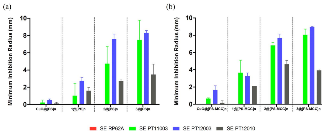
Fig. 5 Normalized antibacterial activity of [\text{PS}]_n (a) and [\text{PS-MCC}]_n (b) films doped with 5% of CuO ( \text{CuO}@\text{[PS]}_n and \text{CuO}@\text{[PS-MCC]}_n ), 1 ( 1@\text{[PS]}_n and 1@\text{[PS-MCC]}_n ), 2 ( 2@\text{[PS]}_n and 2@\text{[PS-MCC]}_n ), and 3 ( 3@\text{[PS]}_n and 3@\text{[PS-MCC]}_n ) against four strains of S. epidermidis (SE), namely one reference strain (RP62A) and three clinical isolates (PT11003, PT12003, and PT12010). Given insusceptibility of RP62A, the corresponding data do not appear in diagrams.
