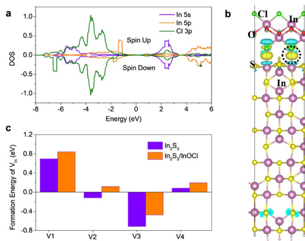
Fig. 3 (a) DOS of In and Cl nearby for the InOCl dissociation on the \beta\text{-In}_2\text{S}_3 (110) surface. The positive and negative values represent spin-up and spin-down states, respectively. (b) The electron density difference of the InOCl/ \beta\text{-In}_2\text{S}_3 (110) interface. The value of the isosurface is 0.0005 \text{ e} \text{ \AA}^{-3} . Yellow color and sky-blue colors represent the electron density increase and decrease, respectively. (c) The formation energy of a 4-fold In vacancy in \beta\text{-In}_2\text{S}_3 (110) with or without InOCl.
