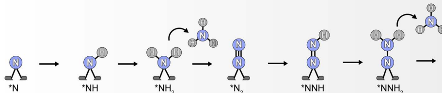
Fig. 1 Common reaction mechanisms for eNRR. (a) Dissociative mechanism. (b) Associative distal mechanism. (c) Associative alternating mechanism. (d) Enzymatic mechanism. (e) Mars–van Krevelen mechanism.
