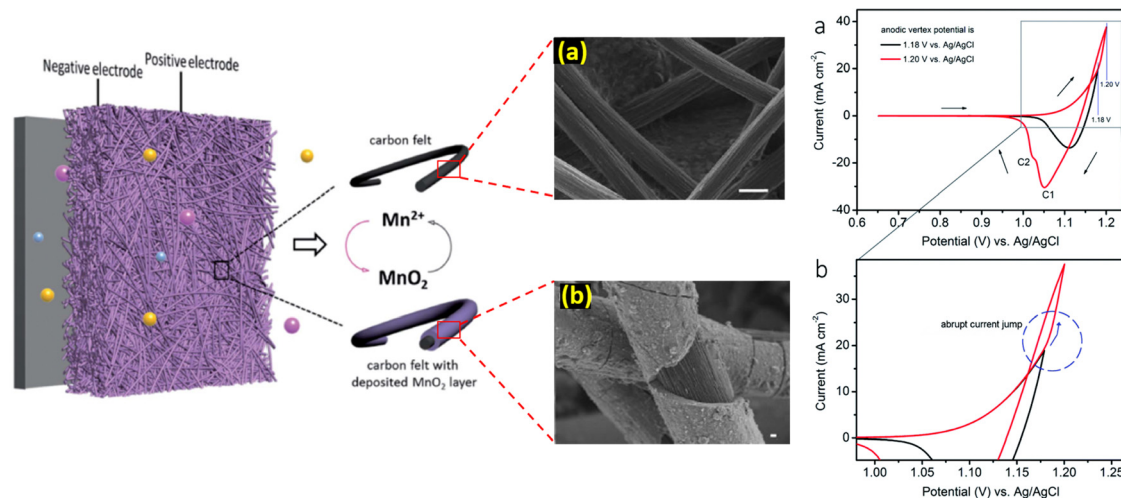
Fig. 3 Understanding the mechanism of Mn 2+ /MnO 2 redox chemistry and the corresponding cyclic voltammogram profile (reproduced from ref. 33 with permission from The Royal Society of Chemistry) (reproduced from ref. 34 with permission from The Royal Society of Chemistry).
