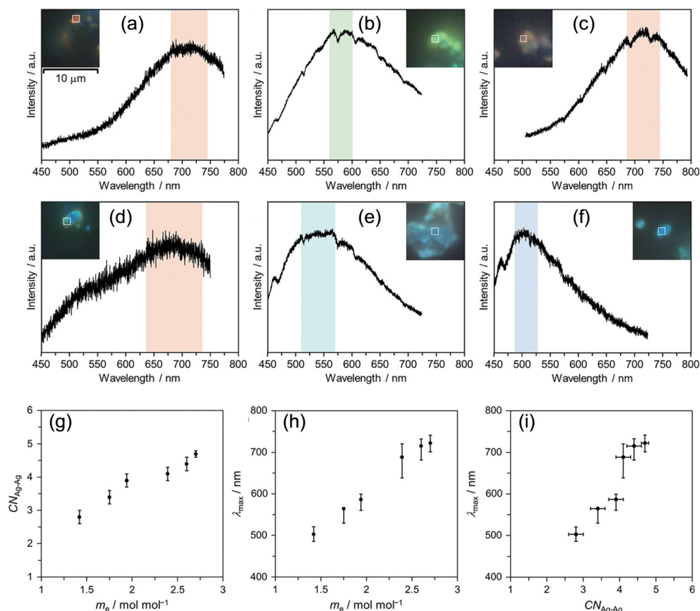
Fig. 11 PL images and spectra of (a) \text{II}_{\text{KMo}}(60, 60) , (b) \text{II}_{\text{KW}}(60, 60) , (c) \text{II}_{\text{NH}_4\text{Mo}}(120, 60) , (d) \text{II}_{\text{KMo}}(1, 60) , (e) \text{II}_{\text{KW}}(1, 60) , and (f) \text{II}_{\text{NH}_4\text{Mo}}(5, 60) . Each spectrum is the sum of PL emitted from the area indicated by the white open square. (g) \text{CN}_{\text{Ag-Ag}} vs. m_e (number of transferred electron), (h) \lambda_{\text{max}} vs. m_e , and (i) \lambda_{\text{max}} vs. \text{CN}_{\text{Ag-Ag}} . The error bar of \lambda_{\text{max}} is estimated by extracting the top 10% intensity range from the smoothed PL spectrum drawn by a moving average of five measurement points. Reprinted with permission from Haraguchi et al. Copyright 2023 Wiley-VCH.
