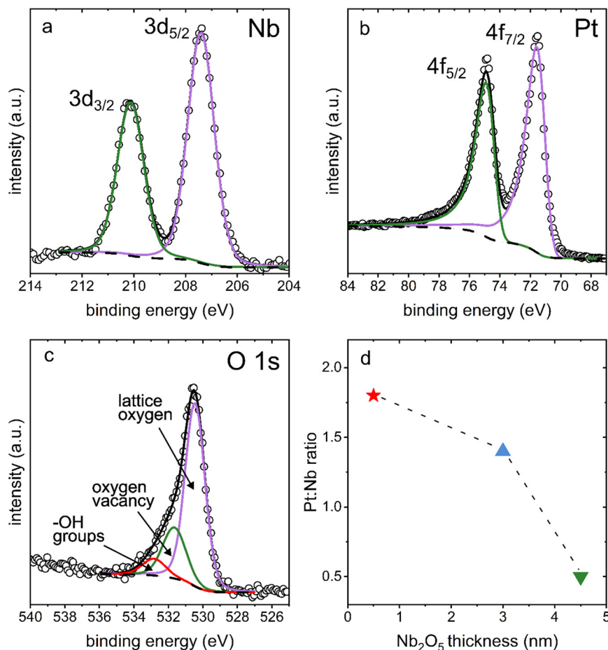
Fig. 4 High-resolution X-ray photoelectron spectroscopy (XPS) analyses of the (a) Nb 3d, (b) Pt 4f, and (c) O 1s species present in the nanostructured Pt samples coated with a 3 nm thick film of \text{Nb}_2\text{O}_5 . Raw data are plotted as hollow circles, and the overall fits are plotted as solid lines. (d) Plot of the ratio of Pt : Nb as calculated from survey spectra of the electrodeposited Pt after coating with (red star) 0.5 nm, (blue triangle) 3 nm, and (green triangle) 4.5 nm thick films of \text{Nb}_2\text{O}_5 . The dashed line was added to draw notice to the non-linearity of the three plotted Pt : Nb ratios.
