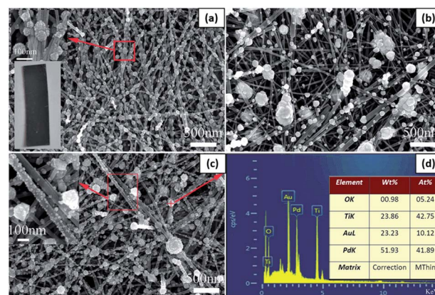
Fig. 9 SEM pictures of (a) Pd@ \text{TiO}_2 , (b) Au@ \text{TiO}_2 and (c) Pd 4 Au@ \text{TiO}_2 . (d) The EDS spectrum for the particle in panel (c) marked with a red "+" symbol. The upper-left and bottom-left insets in panel (a) are the enlarged SEM image of a few NPs and the photograph of Pd@ \text{TiO}_2 , respectively. The inset in panel (c) is the enlarged SEM image for the marked region with a red box. The inset in panel (d) lists the elemental distribution in Pd 4 Au@ \text{TiO}_2 . Adapted with permission from ref. 101. Copyright (2016) Royal Society of Chemistry (RSC).
