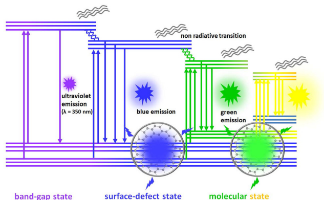
Fig. 12 The fluorescence emission mechanism in multiemission carbon dots is described as individual contributions from the quantum size effect, surface state and molecular state.
