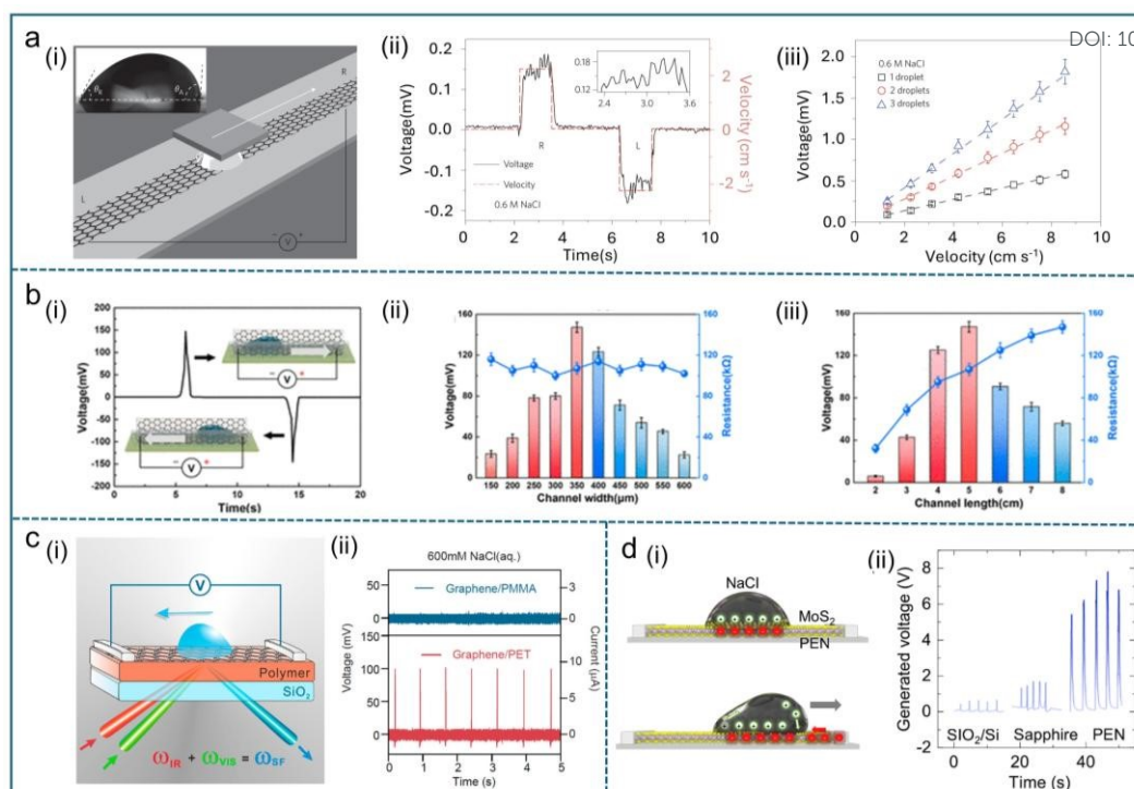
Figure 21. Application of droplet energy generator. a) (i) The droplet slides on the graphene sheet drawn by Si wafer, generating a drag potential. a) (ii) Drawing a droplet from the left end of the graphene strip to the right end and back again generates a voltage of 0.15mV. The reversed droplet velocity will generate a negative output voltage. a) (iii) The voltage induced when moving one, two, and three droplets. The output voltage is proportional to the number of droplets. Reproduced with permission. 274 Copyright 2014, Springer Nature. b) (i) The voltage generated by a 0.6 M NaCl solution when it moves in a graphene microchannel. The voltage direction varies with the flow direction of the droplet. b) (ii - iii) The output voltage of the graphene microchannel device changes at different channel widths and heights. Reproduced with permission. 334 Copyright 2022, American Chemical Society. c) (i) The droplet energy generator consisted of graphene/polymer film on SiO 2 plate. c) (ii) The graphene/PET film can generate 100mV pulse voltage, while it is undetectable on the graphene/PMMA. Reproduced with permission. 336 Copyright 2018, American Chemical Society. d) (i) Mechanisms of electricity generation while the droplet sliding on MoS 2 film. d) (ii) Voltage generated while MoS 2 film underlying on different substrates. Reproduced with permission. 339 Copyright 2020, Elsevier.
