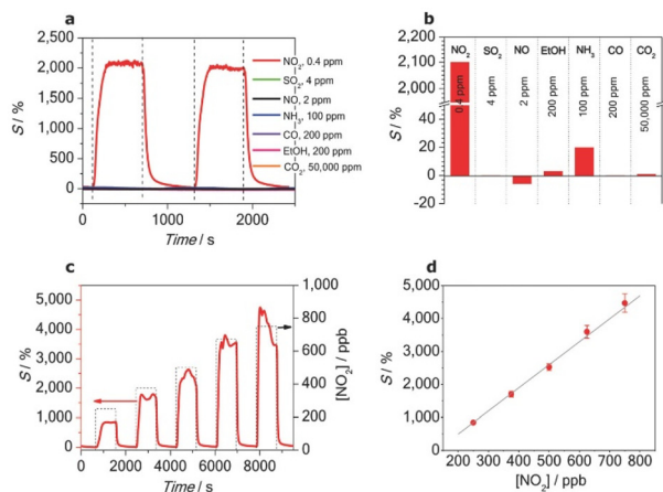
Fig. 7 en-APTAS 1 functionalized \text{SnO}_2 NW sensor measured under solar illumination ( 85 \text{ mW cm}^{-2} ). (a) Pulses of 0.4 ppm \text{NO}_2 , \text{SO}_2 (4 ppm), NO (2 ppm), \text{NH}_3 (100 ppm), ethanol (200 ppm), CO (200 ppm) and \text{CO}_2 (50 000 ppm). (b) Summary of sensitivities towards the tested gases. (c) Sensing response vs. different \text{NO}_2 concentrations ranging from 250 to 750 ppb in synthetic air. (d) Linear behaviour of the sensor response with different \text{NO}_2 concentrations. Reproduced from ref. 48 with permission from Wiley, copyright 2014.
