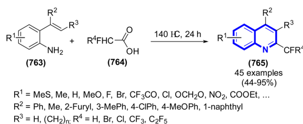
Scheme 216 Synthesis of 2-fluoroalkylated quinolines under catalyst-free conditions.
