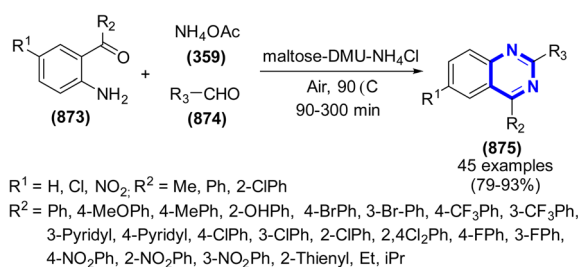
Scheme 249 Synthesis of quinazolines catalyzed by a low melting point mixture.
