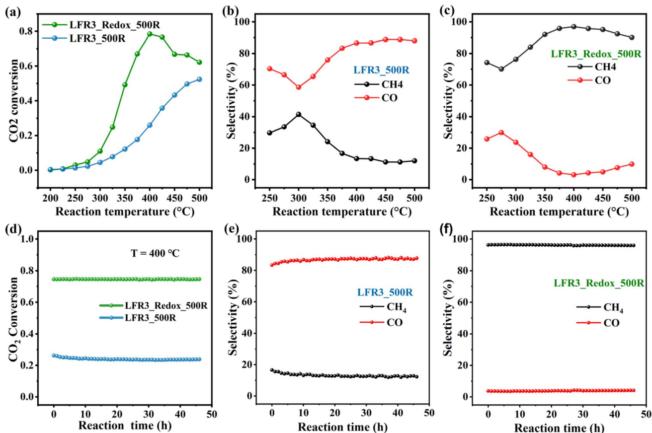
Fig. 6 (a) Activity and (b and c) selectivity of \text{CO}_2 hydrogenation over LFR3_500R and LFR3_Redox_500R as a function of temperature. Long-term stability in terms of (d) activity and (e and f) selectivity of LFR3_500R and LFR3_Redox_500R in the \text{CO}_2 hydrogenation reaction at 400 °C. The feeding gas consists of 4 sccm of \text{CO}_2 and 16 sccm of \text{H}_2 that is balanced by 20 sccm of Ar.
