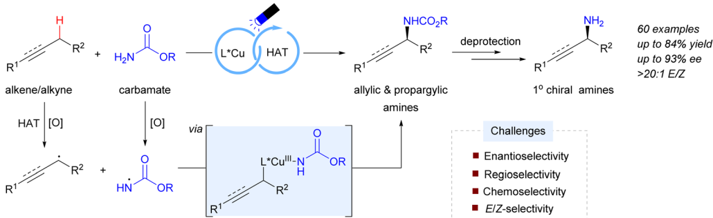
Scheme 1 Catalytic asymmetric allylic C–H amination reactions.
