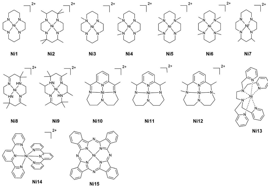
Chart 2 Nickel complexes.
