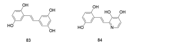
Fig. 13 The chemical structures of inhibitors with diverse mechanisms.
