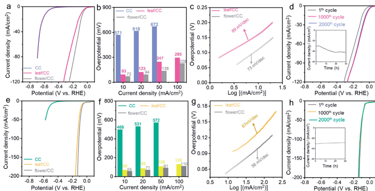
Fig. 3 The comparison of (a) LSVs, (b) overpotentials, (c) Tafel slopes and (d) stability tests for two nanomaterials in HER under neutral conditions with H 2 -saturated phosphate buffer solution. The comparison of (e) LSVs, (f) overpotentials, (g) Tafel slopes and (h) stability tests for two nanomaterials in HER in H 2 -saturated 1.0 M KOH aqueous solution. The scan rate is 5 mV s -1 , and post- i R compensation is applied.
