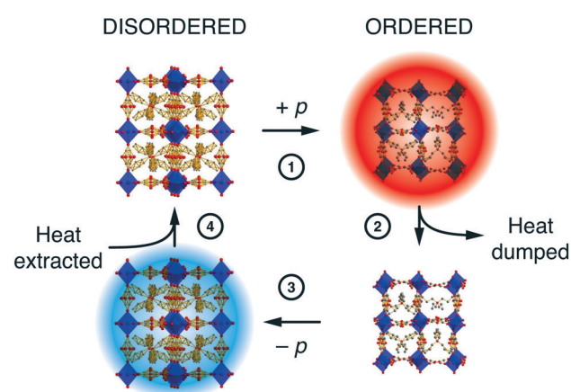
Fig. 5 A simple barocaloric cooling strategy that exploits the pressure-dependence of the order/disorder transition in [NPr 4 ] [Mn(N(CN) 2 ) 3 ]. Starting at ambient conditions where the system is orientationally disordered (top left), ordering is induced by (1) application of pressure (note the change in unit cell dimensions is exaggerated here for effect). The loss of configurational entropy results in heating, and this excess heat (2) is dumped to the environment. (3) Removing the applied pressure forces the system to disorder; the concomitant increase in entropy now requires the system to cool. The cold solid (4) extracts heat from its environment. 74,75 Adapted from ref. 74 with permission from Springer Nature.
