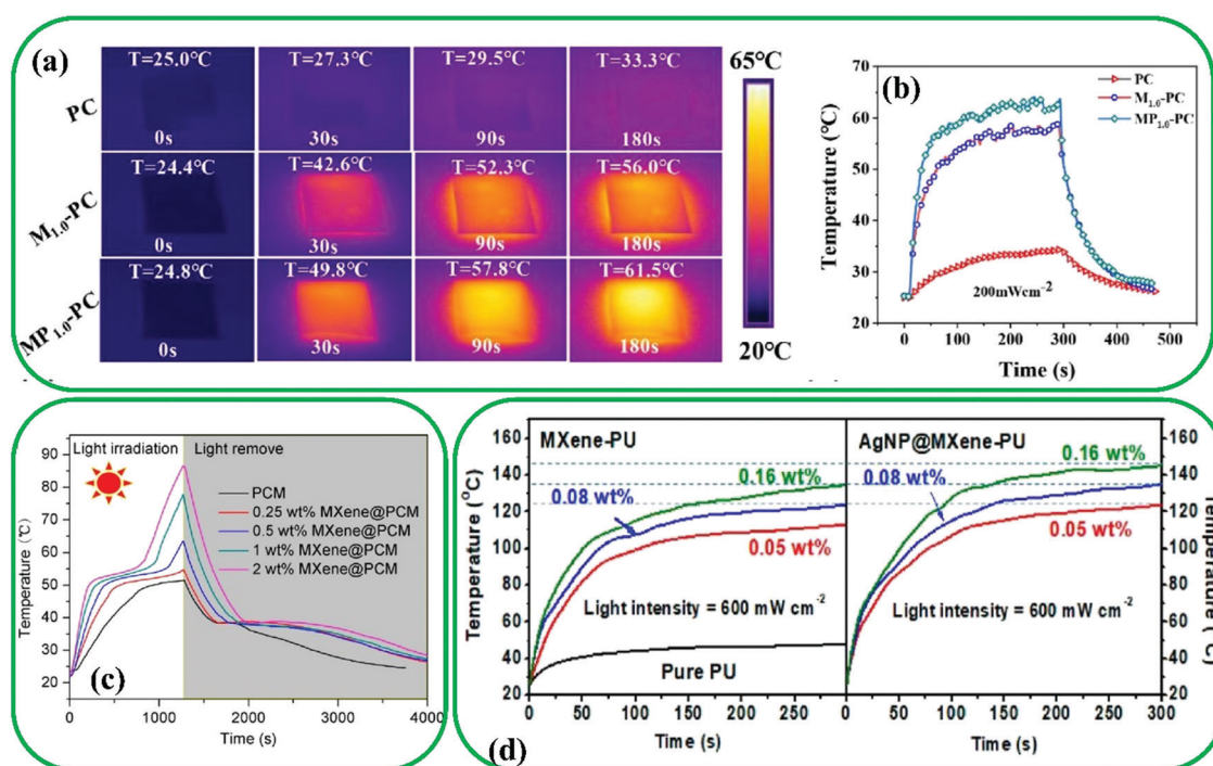
Fig. 20 (a) IR thermal images and (b) surface temperature evolution curves of different MXene@PPy-based films under 200 mW cm^{-2} . Reproduced with permission. 239 Copyright 2021, American Chemical Society. (c) Temperature evolution curves of pristine PCM and MXene@PCM at different concentrations of Ti_3C_2 . Reproduced with permission. 240 Copyright 2020, American Chemical Society. (d) Temperature changes as a function of time for MXene-PU (left) and AgNP@MXene-PU (right) under 600 mW cm^{-2} . Reproduced with permission. 241 Copyright 2019, American Chemical Society.
