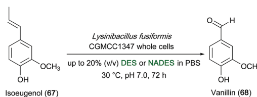
Scheme 26 Bioconversion of isoeugenol ( 67 ) to vanillin ( 68 ) catalyzed by Lysinibacillus fusiformis CGMCC1347 whole cells in DES or NADES mixtures.
