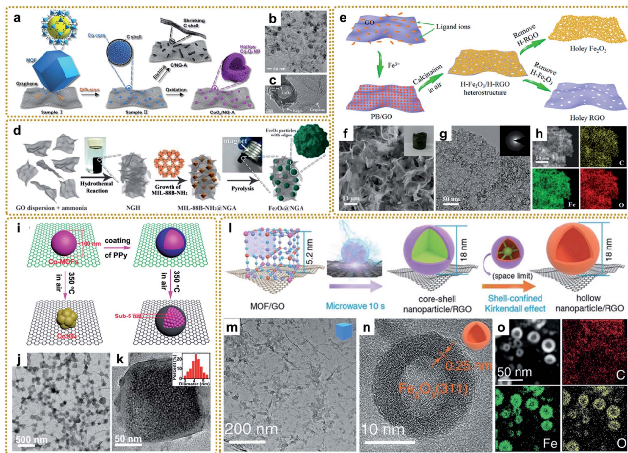
Fig. 7 (a) Schematic of the formation process of CoO x /NG-A and C/NG-A. (b) TEM image of CoO x /NG-A. (c) HRTEM image of the Co 3 O 4 phase in CoO x . Reproduced with permission from ref. 132. Copyright 2017, American Chemical Society. (d) Synthesis process for the Fe 3 O 4 @NGA catalyst. Reproduced with permission from ref. 137. Copyright 2017, Wiley-VCH. (e) Schematic illustration of the synthesis process of the H-Fe 2 O 3 /H-RGO heterostructure. (f) SEM and (g) TEM images, and (h) STEM image and the corresponding elemental mapping images of the H-Fe 2 O 3 /H-RGO. The inset in panel (f) shows the photograph of a monolithic H-Fe 2 O 3 /H-RGO aerogel. The inset in panel (g) shows the SAED pattern of the H-Fe 2 O 3 /H-RGO. Reproduced with permission from ref. 41. Copyright 2018, American Chemical Society. (i) Schematic illustration of the spatially confined pulverization process. (j) TEM image, and (k) HRTEM image of GCP350. The inset of (k) is a histogram of the size distribution of nanocrystals. Reproduced with permission from ref. 42. Copyright 2018, American Chemical Society. (l) Illustration of the synthesis process of hollow nanoparticles/RGO. (m) TEM image of the PB/GO aerogel, (n) HRTEM and (o) STEM images, and elemental mapping images (C, Fe, and O) of S-H-Fe 2 O 3 /RGO. Reproduced with permission from ref. 39. Copyright 2020, Wiley-VCH.
