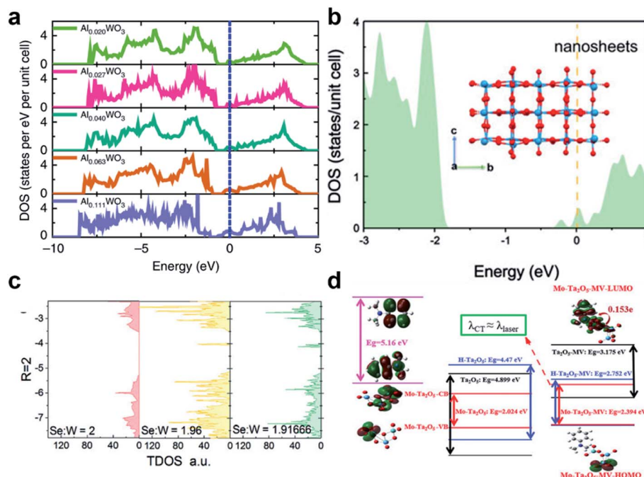
Fig. 7 Manipulation of DOS in semiconductors by defect engineering. (a) DOS of different concentration Al-doped WO 3 . Reproduced with permission from ref. 43. Copyright 2019, Springer Nature. (b) DOS of simulated ultrathin WO 3 nanosheets. Reproduced with permission from ref. 69. Copyright 2021, John Wiley and Sons. (c) TDOS of WSe 2 with different W : Se atomic ratios. Reproduced with permission from ref. 105. Copyright 2018, John Wiley and Sons. (d) Illustrations of CT resonance processes in different MV–Ta 2 O 5 complexes. Reproduced with permission from ref. 25. Copyright 2019, John Wiley and Sons.
