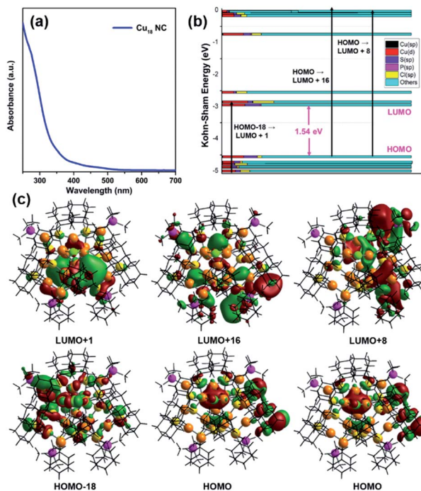
Fig. 6 (a) UV-vis spectrum of the Cu 18 NC dissolved in chloroform, (b) Kohn–Sham molecular energy diagram with the corresponding transitions, and (c) associated frontier molecular orbital diagram. Color legend: Cu, deep orange; S, yellow; P, magenta; Cl, green. All phenyl and adamantane groups are presented in wire-frame.
