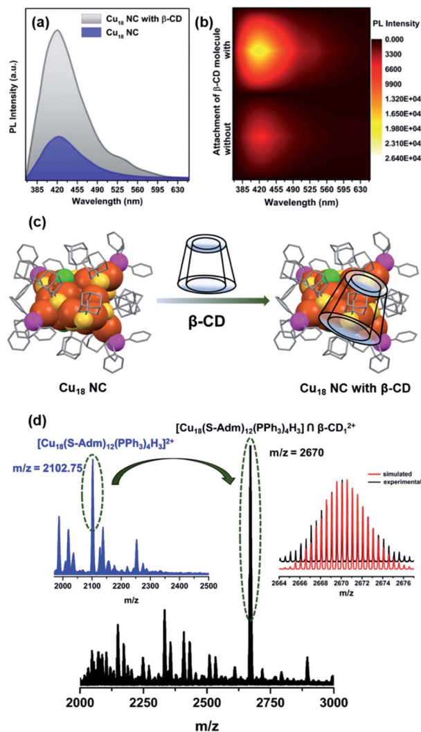
Fig. 7 (a) PL spectra of the Cu 18 NC before and after adduct formation with β-CD. (b) 2-D contour plot of the PL intensity with the number of β-CD molecules attached to the Cu 18 NC. (c) Schematic representation of the host–guest interaction. (d) Positive-mode ESI-MS spectrum of Cu 18 n β-CD 1 . The inset shows the experimental and simulated patterns of the peak corresponding to [Cu 18 (S-Adm) 12 (PPh 3 ) 4 H 3 ] n β-CD 1 2+ which is shifted relative to the initial ESI-MS spectrum of the pure Cu 18 NC. Color legend: Cu, deep orange; S, yellow; P, magenta; Cl, green. All phenyl and adamantane groups are presented in wire-frame.
