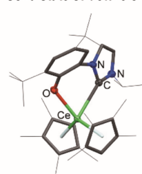
Scheme 1 Syntheses of the complexes examined for C–F bond functionalization in this work (upper) and the solid-state structure of 1-Ce, H omitted for clarity, alongside the ligand variations studied for 1-Ce (lower).
