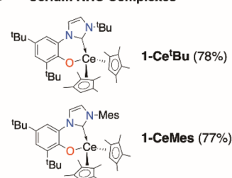
Scheme 1 Syntheses of the complexes examined for C–F bond functionalization in this work (upper) and the solid-state structure of 1-Ce, H omitted for clarity, alongside the ligand variations studied for 1-Ce (lower).
