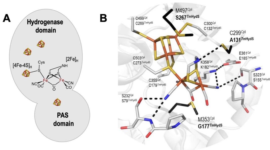
Fig. 1 (A) Arrangement of cofactors in TmHydS. The [4Fe-4S] H clusters are shown as brown and yellow cubes and the [2Fe] H cluster is shown in chemical structure format. (B) Close-up structural view of the H-cluster including the surrounding second coordination sphere amino acids. The structure is of the C. pasteurianum (Cpl) enzyme (PDB ID: 4XDC). 12 Amino acid positions are labelled each with their Cpl (top) and TmHydS (bottom) identities. Amino acids coloured in black (bold) were mutated in this study. The figure was prepared in Pymol. The dashed lines indicate hydrogen bonds between the H-cluster and surrounding amino acids. For an alternative view showing the location of Y223 see Fig. S2A.†
