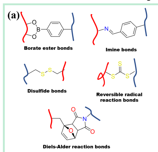
Fig. 14 Different strategies for designing self-healing hydrogels. (a) Chemical crosslinking self-healing mechanisms (b) physically crosslinking self-healing mechanisms.
