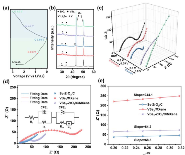
Fig. 6 (a) Discharge/charge curve and corresponding voltage positions of VSe_2-ZrO_2/C/MXene . (b) Ex situ XRD characterizations of the corresponding potential states. (c) EIS plots of VSe_2-ZrO_2/C/MXene at various states in the 40th cycle at 100 mA g^{-1} . (d) Nyquist plots of Se-ZrO_2/C , VSe_2/MXene and VSe_2-ZrO_2/C/MXene after 100 cycles at 100 mA g^{-1} (inset: corresponding equivalent circuit model). (e) Fitted lines of Z' versus \omega^{-1/2} at low frequency for VSe_2-ZrO_2/C/MXene .
