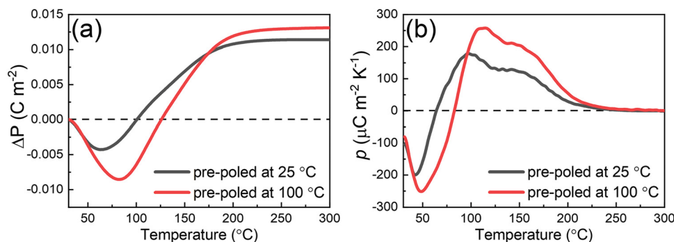
Fig. 6 Temperature-dependent changes in (a) remanent polarization, \Delta P , and (b) pyroelectric coefficient, p , of 0.5 mol% Nb-doped 0.7\text{BF} – 0.3\text{BT} pre-poled at 25 and 100 °C.
