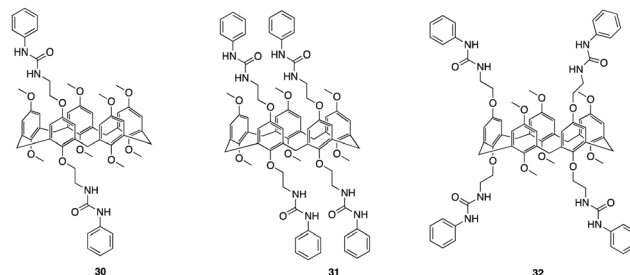
Fig. 17 General structures of urea functionalised pillar[5]arenes 30–32 reported by Al-Azemi and co-workers.
