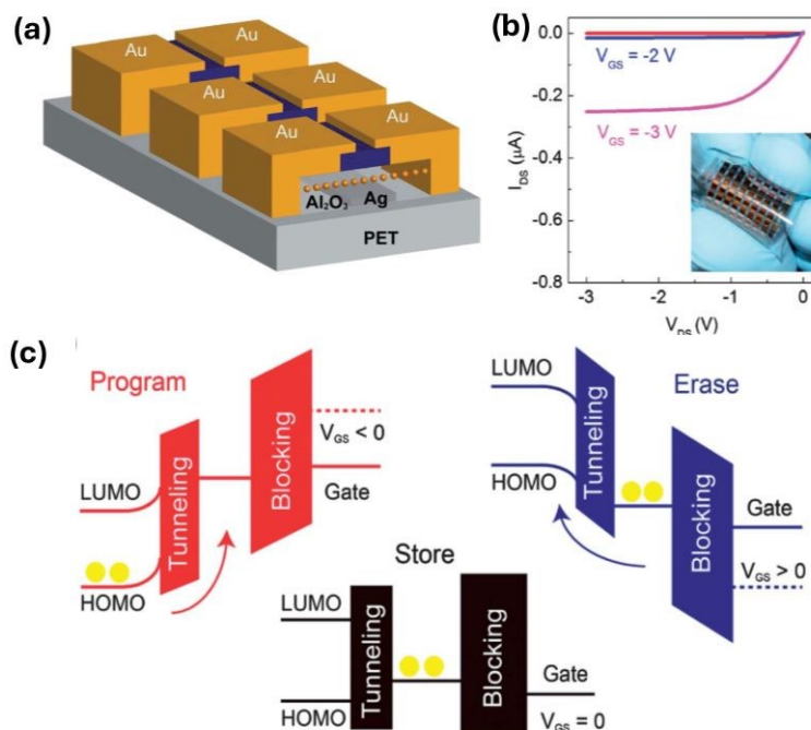
Figure 11: Comprehensive view and characteristics of the flexible memory array. (a) Three-Dimensional Illustration: This panel presents a three-dimensional representation of the flexible memory array, showcasing its structural design and layout. (b) Output Characteristics: The output characteristics of the memory transistors in their programmed state are displayed here. The inset provides an optical image of the flexible memory arrays, giving a visual confirmation of their physical appearance and flexibility. (c) Energy Diagram: This diagram illustrates the energy levels and electron flow within the memory transistor, detailing the charge trapping and release mechanisms that underpin its operation. Reproduced from ref. [49] with permission from [RSC Publishing], copyright [2013].
