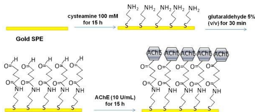
Figure 21. Assembly process of the AChE Biosensor. Reproduced from ref. [67] with permission from [Elsevier], copyright [2013].
