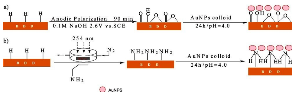
Figure 16. The self-assembly of Au-NPs onto BDD surfaces: (a) hydroxyl/oxide-terminated activated BDD surface, and (b) amine-terminated activated BDD surface. Reproduced from ref. [60] with permission from [ACS Publications], copyright [2006].
