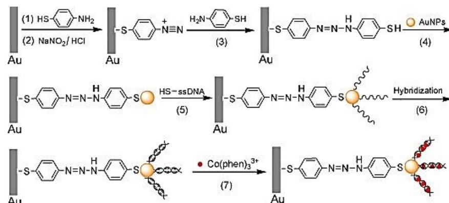
Fig. 22. Fabrication of DNA biosensor. Reproduced from ref. [68] with permission from [Elsevier], copyright [2005].
