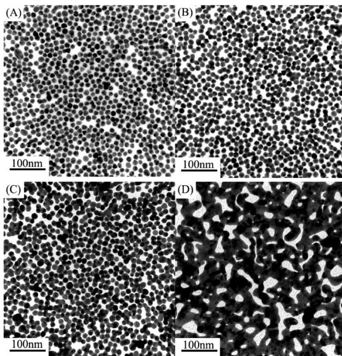
Figure 3. TEM images of Au-NP monolayers: (A) without aging, (B) aging for 3 days, (C) aging for 7 days, and (D) aging for 10 days. Reproduced from ref. [28] with permission from [IOP Publishing], copyright [2010].
