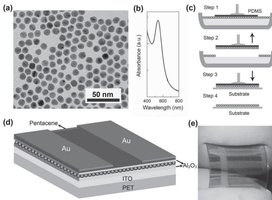
Figure 13 presents: (a) TEM image of 10 nm Au NPs coated with DDT. (b) UV-visible absorption spectra of Au-NPs in toluene. (c) Schematic process of forming NPs array on a substrate. (d) 3D schematic of the memory device architecture. (e) Optical photo of the fabricated flexible memory device. Reproduced from ref. [50] with permission from [Wiley], copyright [2012].
