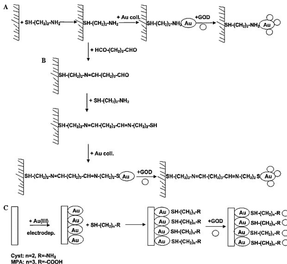
Fig. 20. Preparation strategies for glucose oxidase biosensors using gold nanoparticle-modified electrodes: (A) GO_x/Au_{coll}-Cyst-AuE , (B) GO_x/Au_{coll}-Cyst/Cyst-AuE , (C) GO_x/Cyst-nAu-GCE or GO_x/MPA-nAu-GCE . Reproduced from ref. [66] with permission from [Elsevier], copyright [2005].
