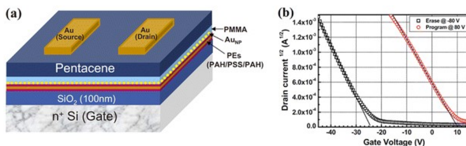
Figure 14: (a) Device Structure and (b) Program/Erase Characteristics of Organic Transistor-Based Nano-Floating-Gate Memory Devices. Reproduced from ref. [51] with permission from [AIP Publishing], copyright [2010].
