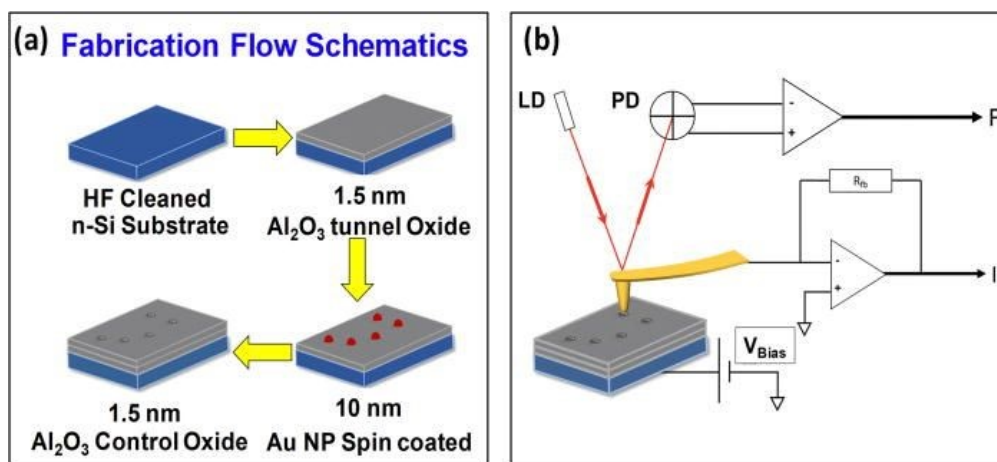
Figure 9. (a) Fabrication process for nanomemory devices and (b) the circuit setup for probing a single Au-NP using conductive atomic force microscopy (C-AFM). Reproduced from ref. [47] with permission from [AIP Publishing], copyright [2020].
