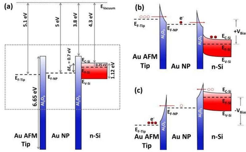
Figure 10 Energy band diagram for NP-based memory operations: (a) Energy levels of materials at zero bias, with no contacts and no charge in the Au-NP. (b) Electron energy levels during charge injection into the Au-NP under positive bias. (c) Electron energy levels during discharge of the Au-NP under negative bias. Diagrams (b) and (c) correspond to the dashed rectangle in (a). Reproduced from ref. [47] with permission from [AIP Publishing], copyright [2020].
