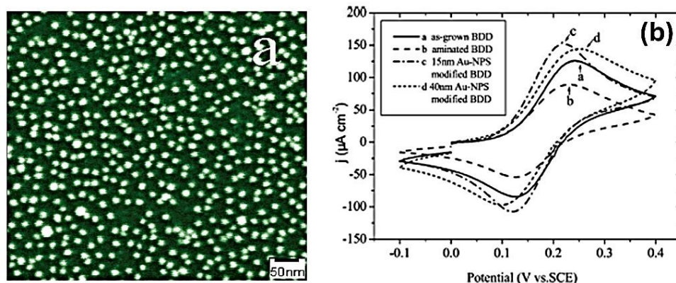
Figure 17: (a) SEM images of amine-terminated BDD surfaces exposed to 15 nm Au-NP solutions for 6 hours., (b) CVs of 1 mM \text{Fe}(\text{CN})_6^{3-/4-} in 0.1 M \text{Na}_2\text{SO}_4 at 50 mV/s for (a) as-grown BDD, (b) amine-terminated BDD, (c) 15 nm Au-NPs on BDD, and (d) 40 nm Au-NPs on BDD. Reproduced from ref. [60] with permission from [ACS Publications], copyright [2006].
