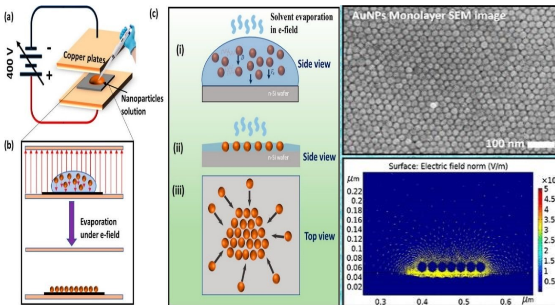
Figure 4 outlines the Au-NP deposition process on a silicon substrate. (a) Shows the experimental setup for NP deposition under an electric field. (b) Provides a schematic of the monolayer formation of Au-NPs on the substrate. (c) Depicts both side and top views of the monolayer formation influenced by the electric field and NP diffusion, (d) SEM image and (e) COMSOL simulation of electric field effect on the negatively charged Au-NPs. Reproduced from ref. [31] with permission from [ACS Publications], copyright [2023].
