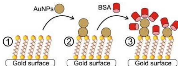
Figure 24. Fabrication Process of the SPR Biosensor: Formation of 1,10-DDT SAM on Gold, Chemisorption of Au-NP to 1,10-DDT SAM, Immobilization of BSA on AuNP. Reproduced from ref. [71] with permission from [Elsevier], copyright [2009].
