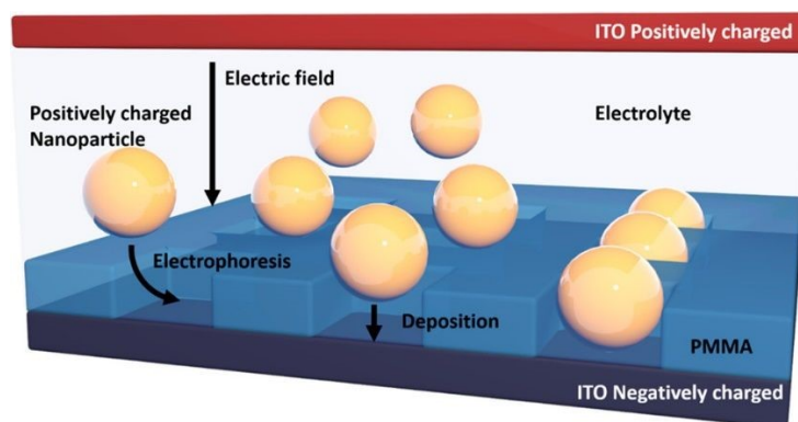
Figure 6. Schematic of the EPD process showing nanospheres deposited onto EBL fabricated ITO-PMMA template. Reproduced from ref. [45] with permission from [ACS Publications], copyright [2018].
