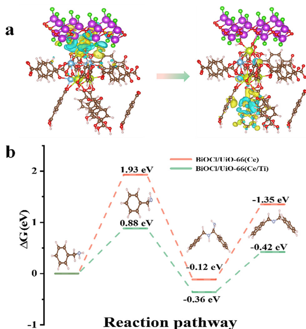
Fig. 8 Differential charge densities (DCDs) of (a) BiOCl/Uio-66(Ce/Ti) before and after the adsorption of BA; (b) free energy diagrams for the adsorption and photoconversion of BA on BiOCl/Uio-66(Ce/Ti) and BiOCl/Uio-66(Ce). Purple, green, yellow, blue, brown, red, pink, and blue grey atoms are Bi, Cl, Ce, Ti, C, O, H, and N respectively.
