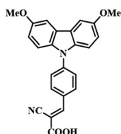
(31) Cz-CA (PCE=20.17%)
