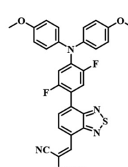
(30) 2FMPA-BT-CA (PCE=21.68%)
