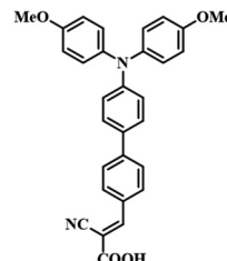
(36) MPA-Ph-CA (PCE=22.53%)
