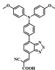
(28) MPA-BT-CA (PCE=21.24%)
