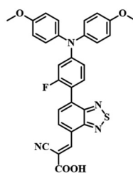
(29) FMPA-BT-CA (PCE=22.37%)
