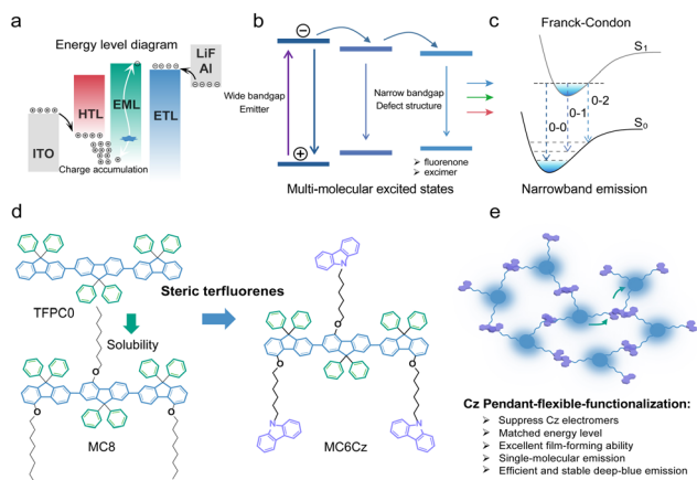
Scheme 1 Molecular design principle of unsymmetrical substituted steric terfluorenes via pendant side-functionalization. (a) Energy level diagram of traditional OLED based on terfluorenes. 11,29 (b) Undesirable energy transfer from wide bandgap emission center to narrowband defect structure, which results in a low efficiency and color purity of deep-blue emission. 30 (c) To suppress the formation of the charge transfer (CT) state can reduce the structural distortion and present a narrowband emission. The introduction of steric hindrance groups inhibits molecular aggregation and induces narrowband emission. 31 (d) Different pendants of steric terfluorenes. Schematic diagram of unsymmetrical substitution of steric terfluorenes via carbazole pendant functionalization at 4-position. (e) Efficient intermolecular charge transport in the Cz pendant functionalized terfluorene. The pendant Cz group at the unsymmetrical 4-site substitution of fluorene monomers can act as a charge transport station to enhance the film conductivity, although there is an extremely weak intermolecular \pi interaction and electron coupling.
