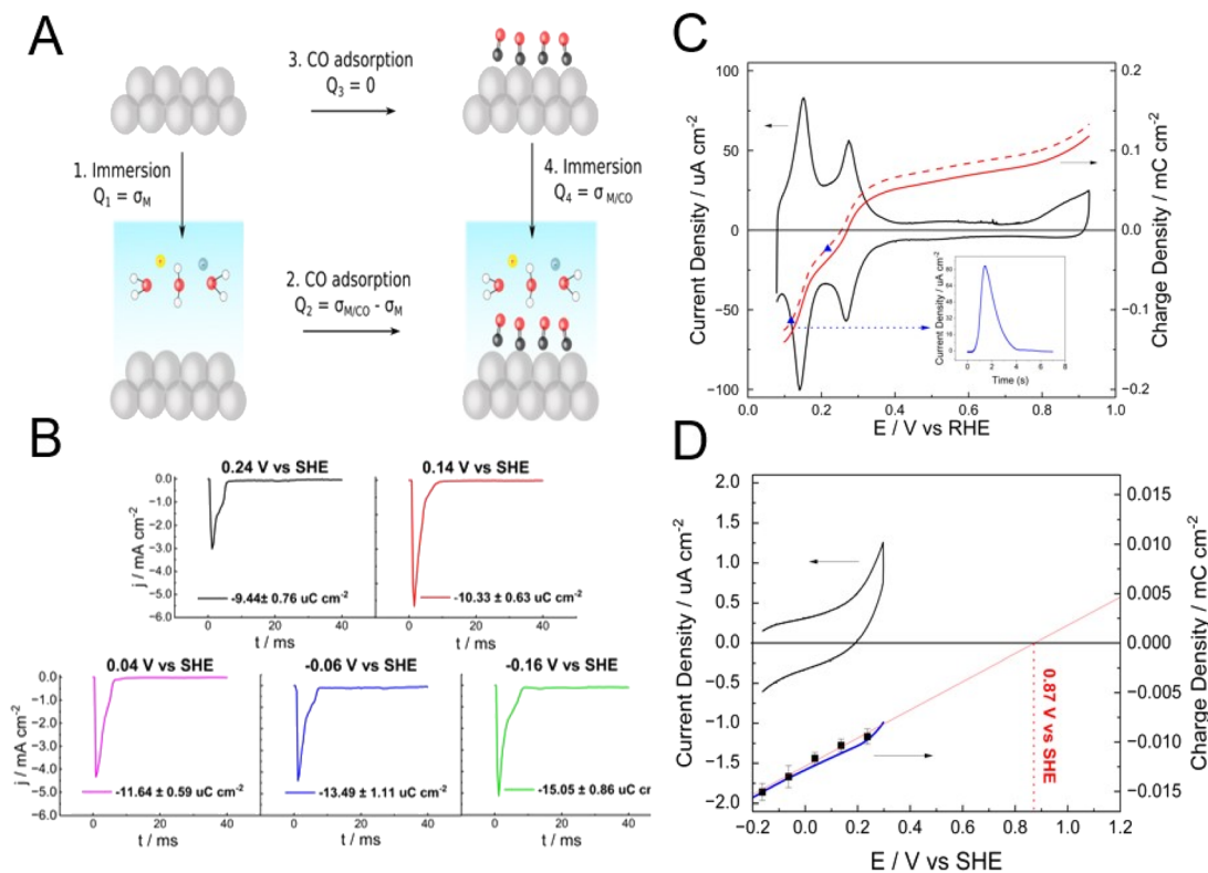
Fig. 4 (A) Schematic description of the immersion (Arrow 1) and CO-charge displacement (Arrow 2) methods for the determination of the pzfc. Arrow 4 corresponds to the determination by the immersion method of the pzfc of an adlayer-covered electrode, a CO adlayer in this example (B) current transients measured during the potentiostatic immersion of a CO-covered Pt electrode in 0.1 M acetate buffer (pH 4.76) at 0.24 (black), 0.14 (red), 0.04 (purple), -0.06 (blue) and -0.16 \text{ V vs. SHE} . The charge resulting from integrating each of the current transient is also provided. (C) CV at 50 \text{ mV s}^{-1} of polycrystalline Pt in 0.1 M acetate buffer (pH 4.76, black line) and charge density vs. potential curves (red lines) obtained by integrating the CV using the charge obtained from a CO-charge displacement experiment at 0.12 \text{ V vs. RHE} (see inset) as the integration constant, before (dashed line) and after (solid line) correction with the charge present on the CO-covered Pt electrode at that potential as obtained from the corresponding potentiostatic immersion experiments shown in (B). The blue dots on the red dashed line correspond to the charge measured in CO-charge displacement experiments at 0.12 and 0.22 \text{ V vs. RHE} , illustrating the internal consistency of the experiments. The uncorrected and corrected pzfc's resulting from these curves are 0.254 and 0.270 \text{ V vs. RHE} , respectively. (D) Cyclic voltammogram (black line) at 50 \text{ mV s}^{-1} of a CO-covered Pt electrode in 0.1 M acetate buffer (pH 4.76) and charge density vs. potential curve (blue line) obtained by integrating the CV using the charge obtained from a potentiostatic immersion experiment at -0.16 \text{ V vs. SHE} as the integration constant. The black square symbols correspond to the charge density present of the CO-covered Pt electrode at the corresponding potential as obtained from the potentiostatic immersion transients in (B). The red solid line is an extrapolation of the charge density vs. potential curve to \sigma = 0 and yields a pzfc for the CO-covered polycrystalline Pt electrode of 0.87 \text{ V vs. SHE} .
