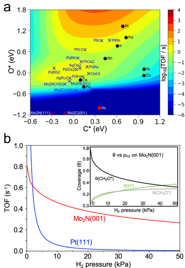
Fig. 5 Screening of catalysts for alcohol dehydrogenation. (a) Turnover frequency of 2-octanol dehydrogenation to 2-octanone as a function of C and O adsorption energy. (b) Predicted turnover frequency of methanol dehydrogenation on Pt(111) and \beta -Mo 2 N(001) from microkinetic modelling of H 2 co-feed at 453 K and p_{\text{CH}_3\text{OH}} = 14 kPa. Inset shows change in coverage of certain intermediates. Reprinted from ref. 80 with permission from Springer Nature, Copyright 2021.
