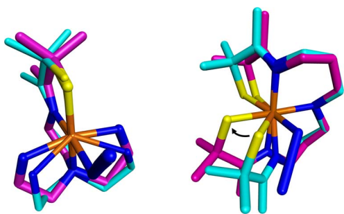
Fig. 12 Visualization of experimentally obtained structural changes that occur upon oxidation and binding of a sixth ligand, azide. Left: [Fe^{II}(S^{Me_2}N_4(tren))]^+ ( 4 , cyan) 36 to [Fe^{III}(S^{Me_2}N_4(tren))N_3] (magenta). 37 Right: [Fe^{II}(S_2^{Me_2}N_3(Pr,Pr))] ( 1 , cyan) 22 and [Fe^{III}(S_2^{Me_2}N_3(Pr,Pr))(N_3)] (magenta). 31 Depiction utilized previously reported crystallographically determined structures.
