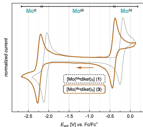
Fig. 3 CV of [\text{Mo}(t^{\text{Bu}}\text{diket})_3] ( 3 ) (1 mM, solid line) and [\text{Mo}^{\text{Me}^e\text{diket}}_3] ( 1 ) (1 mM, dashed line) in \text{TBAPF}_6/\text{MeCN} (0.1 M) at a scan rate of \nu = 100 \text{ mV s}^{-1} .
