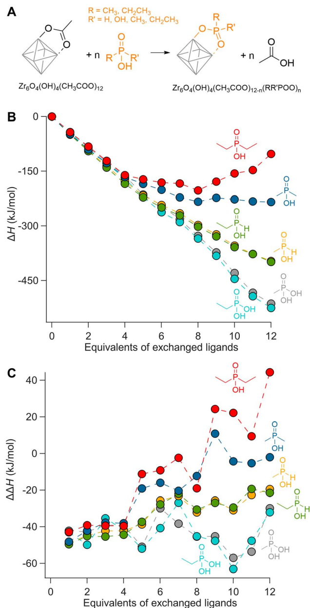
Fig. 1 (A) Scheme representing the exchange of acetate ligands for phosphorus-based ligands on a fully bridged Zr_6 cluster. (B) Enthalpy of ligand exchange reactions as a function of equivalents of exchanged ligands, \Delta H . (C) The enthalpy change for every step, \Delta\Delta H .
