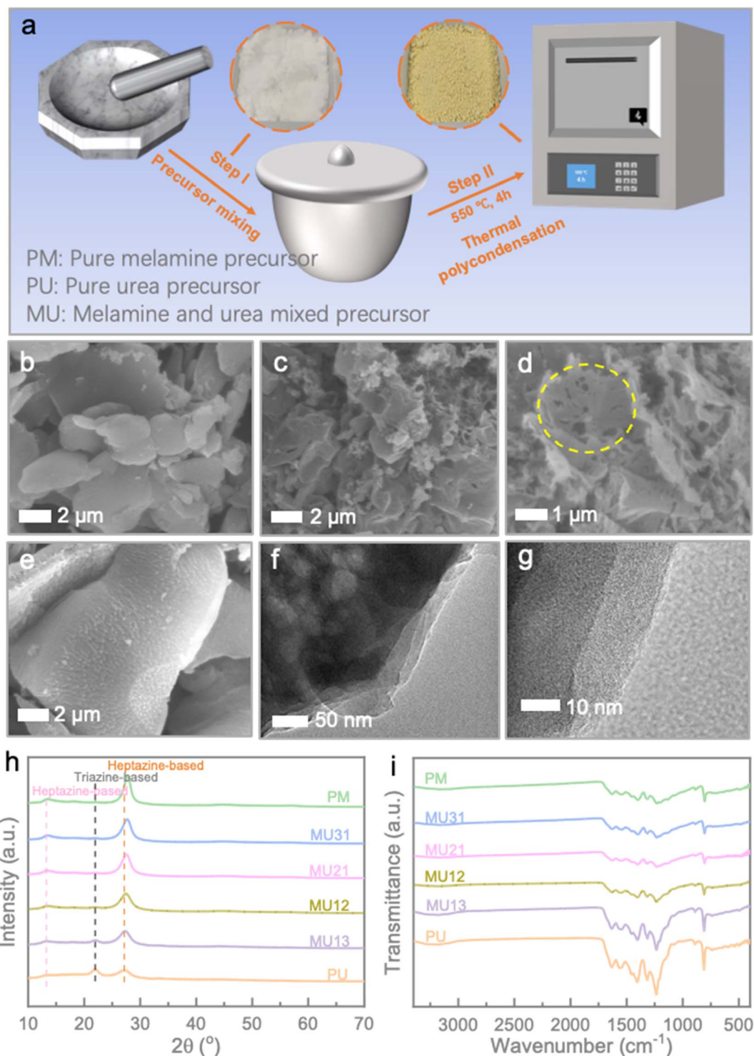
Fig. 1 (a) Schematic illustration of the synthesis of the different g-C 3 N 4 -based samples. SEM images of (b) PM, (c and d) PU, and (e) MU21. (f) and (g) TEM images of MU21 at low and high magnifications. (h) XRD patterns and (i) FT-IR curves of synthesized samples.
