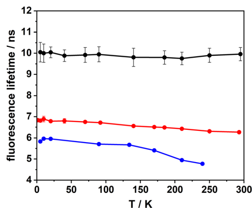
Fig. 4 Temperature dependence of the fluorescence lifetime. Black circles: DBT-d 20 in Zeonex, bulk sample; red circles: DBT-h 20 in Zeonex, bulk sample; blue circles: DBT-h 20 in Zeonex, single molecule. The drawn lines are guides to the eye only.
