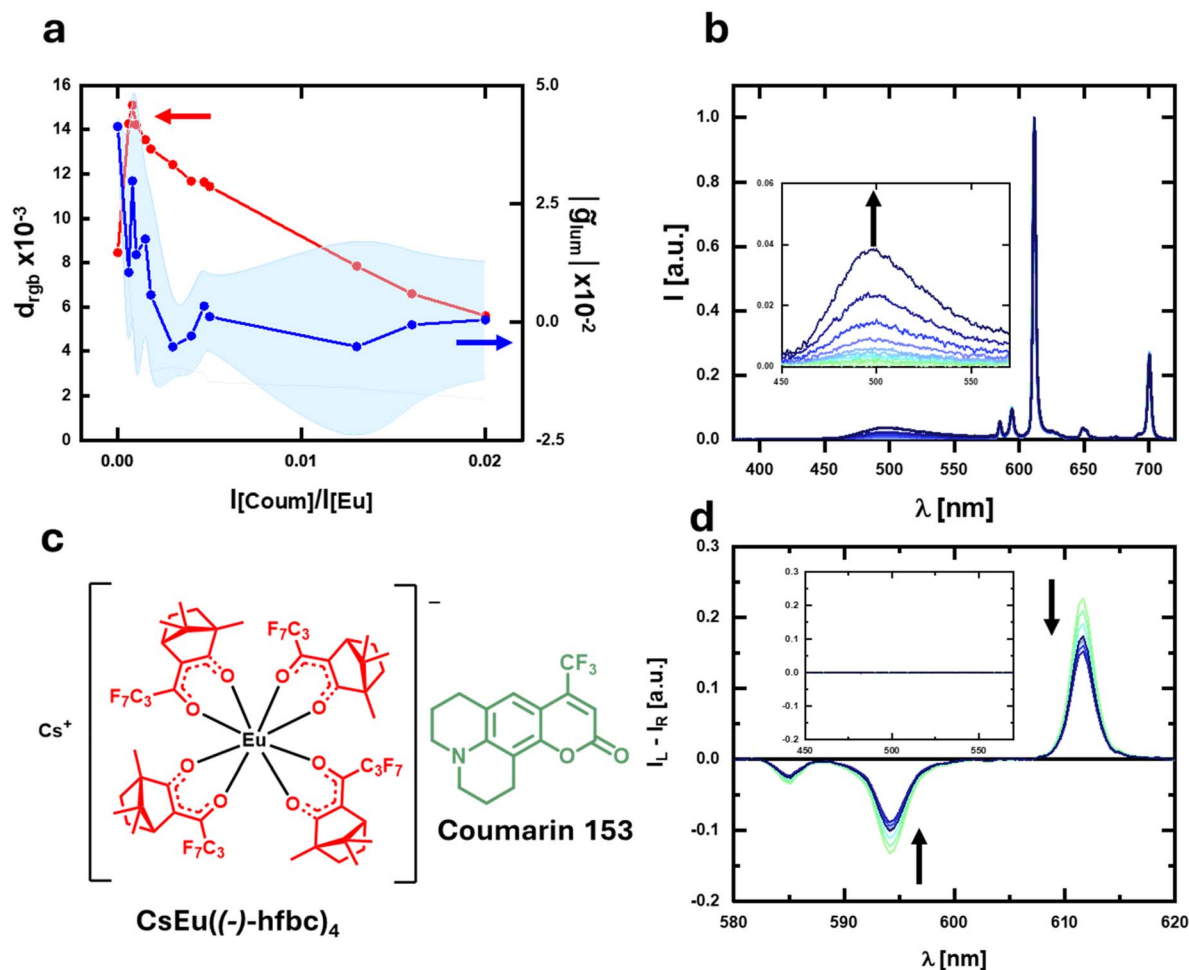
Fig. 4 (a) Plot of d_{rgb} (red) and \tilde{g}_{lum} (blue) for a solution of CsEu((–)-hfbfc) 4 containing increasing amounts of coumarin 153. (b) Emission and (d) corresponding CPL spectra of the solution of CsEu((–)-hfbfc) 4 containing increasing amounts of coumarin 153; the CPL spectra are normalized by the integral of the corresponding total emission spectrum. (c) CsEu((–)-hfbfc) 4 and coumarin 153.
