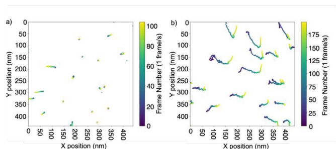
Figure 3. Scatter plots of the trajectories of the center position of AuNP@polyA. The center position of each particle is tracked across a time series of HAADF-STEM images with an electron dose of 20 \text{ e}^-/\text{\AA}^2 per frame (a) and 50 \text{ e}^-/\text{\AA}^2 per frame (b). When the electron dose is low, AuNP@polyA dimers move as stable units (a), whereas for the higher
