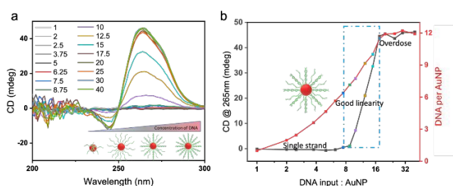
Figure 8. a) CD spectra of AuNP@polyA prepared at different polyA/AuNP ratio. b) Correlation between the number of polyA strands on AuNPs and CD intensity at 265 nm.
