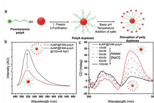
Figure 6. Schematic illustration of the behavior of AuNP@polyA duplexes in the presence of added NaCl. b) Fluorescence spectra of AuNP@FAM-polyA before and after addition of NaCl (100 mM). c) CD spectra of AuNP@polyA at different NaCl concentrations, as labeled.
