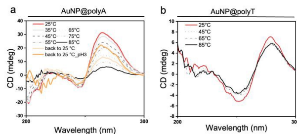
Figure 7. CD spectra of at different temperatures for AuNP@polyA (a) and AuNP@polyT (b).
