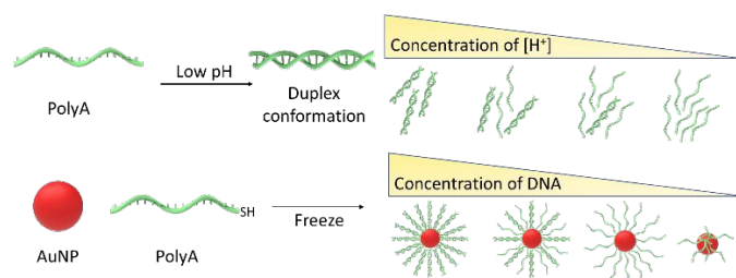
Scheme 1. a) Graphical illustration of secondary structures of polyA at different pH values. b) Graphical illustration of AuNP@polyA, at different DNA concentrations on the gold surface.
