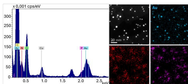
Figure 4. EDX spectra from AuNP@polyA in dried condition, confirming the presence of N and P (from polyA) around AuNPs.
