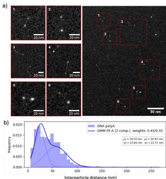
Figure 2. a) HAADF-STEM images of AuNP@polyA in liquid environment, showing the presence of dimers and individual particles. b) Two-component Gaussian mixture model (GMM) showing the presence of AuNP@polyA duplexes and single AuNP@polyA.
