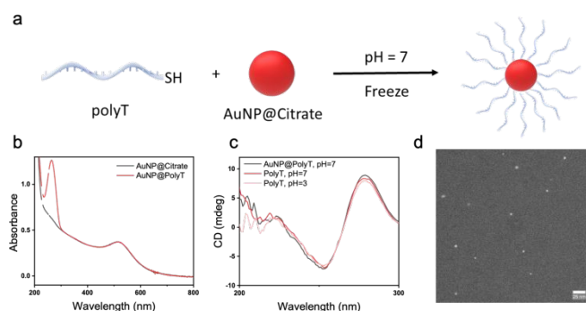
Figure 5. Schematic illustration of AuNP@polyT conjugates. b) UV-Vis spectra of AuNP@citrate and AuNP@polyT. c) CD spectra of AuNP@polyT at pH = 7 (black), polyT (red) at pH = 7 and polyT (pink) at pH = 3. d) Representative liquid-phase TEM image of AuNP@polyT.
