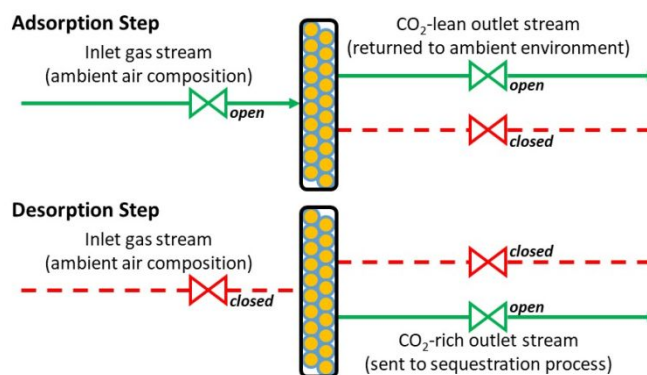
Figure 4: Schematic overview of our idealized adsorption/desorption cycle process used to investigate core-shell MOF candidates. We assume 100% evacuation of adsorbed gases during the desorption step, which can
