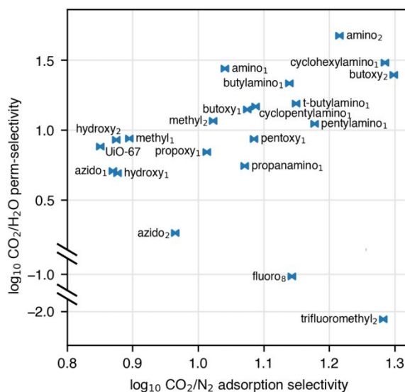
Figure 9: CO 2 / H 2 O perm-selectivity (higher values indicate better performance as a shell) vs CO 2 / N 2 adsorption selectivity (higher values indicate better performance as a core) for selected MOFs.
