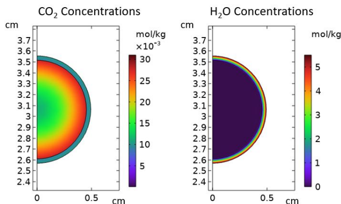
Figure 10: CO 2 concentrations (left) and H 2 O concentrations (right) in a simulated amino 1 ◊methyl 2 spherical pellet at t = 990 seconds.
