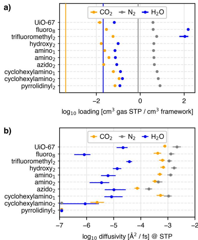
Figure 7: (a) Gas loadings of CO 2 , N 2 and H 2 O for selected MOFs based on UiO-67. Vertical lines are the amount of each gas in the atmosphere. (b) Diffusivities of CO 2 , N 2 and H 2 O for selected MOFs based on UiO-67, with error bars to 95% confidence interval.
