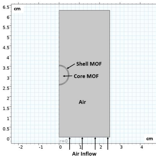
Figure 6: Setup of COMSOL Multiphysics® model of a single core-shell spherical pellet. Air flows in from the bottom over a 0.453 cm radius core + 0.04 cm thick shell pellet.
