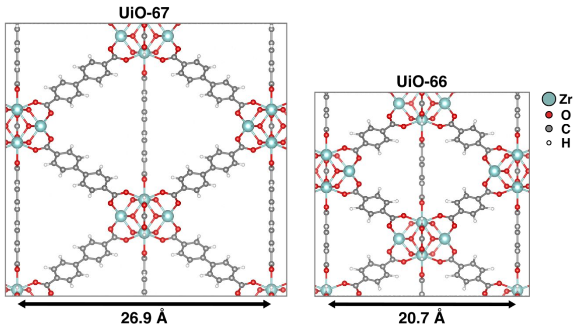
Figure 2: UiO-67 ( left ) and UiO-66 ( right ) structures showing biphenyl and phenyl ligands.
