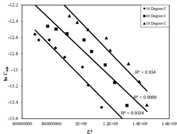
Fig. 9 D–R adsorption isotherm for the Rose Bengal (pH = 7.2)–bottom ash (0.50 g, mesh size = 100 BSS) system at different temperatures.
