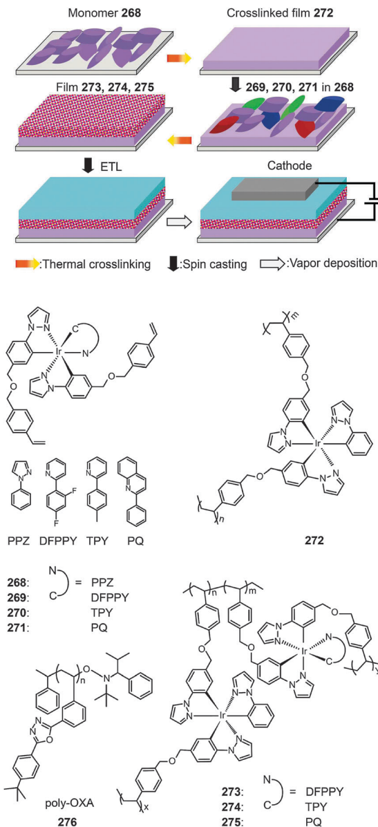
Fig. 18 procedure of solution-processed multi-layer devices on the basis of crosslinkable monomers 268–271 and the corresponding crosslinked polymers 272–275 . (Reproduced with permission from ref. 116. Copyright 2009, Wiley-VCH Verlag GmbH & Co. KGaA.)
