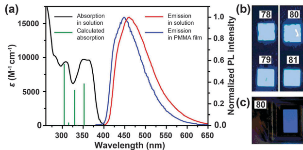
Fig. 7 (a) Absorption and photoluminescence spectra of 78 and 79 . (b) Photographs showing electroluminescent devices derived from 78 – 81 under UV irradiation. (c) Photograph showing electroluminescence emission of the device based on 80 . (Reproduced with permission from ref. 41. Copyright 2011, Royal Society of Chemistry.)
