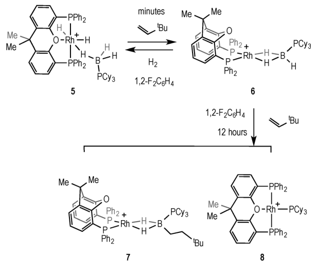
Scheme 9 Formation of 6 , 7 and 8 . [BAR^F_4]^- anions are not shown.
